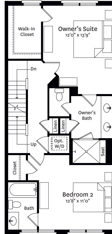
THIRD LEVEL
